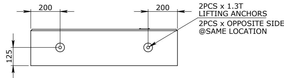
END VIEW
