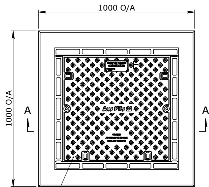
COVER AND FRAME SOLID 600x600 1 PART CLASS D (CRS66D)
