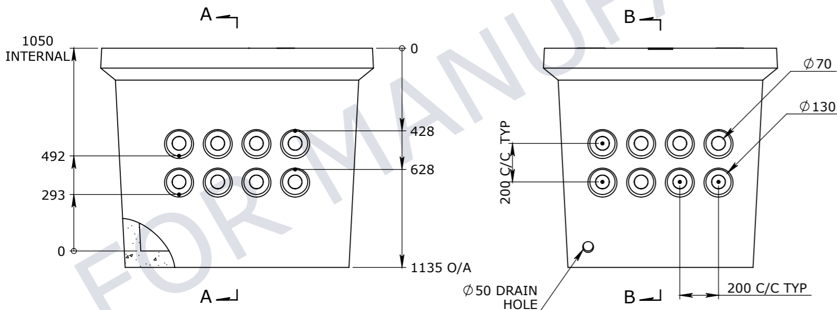
ELEVATION VIEW
