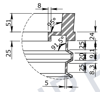
SCALE 1:5 DETAIL D
