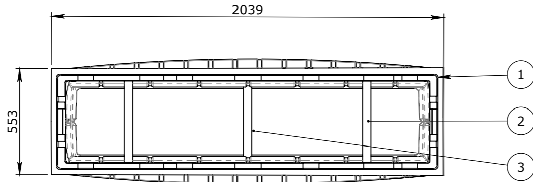
PLAN VIEW
