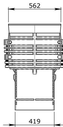
END VIEW
