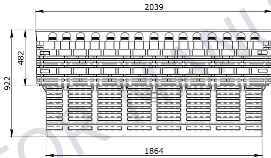
ELEVATION VIEW
