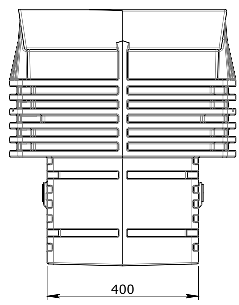
END VIEW
