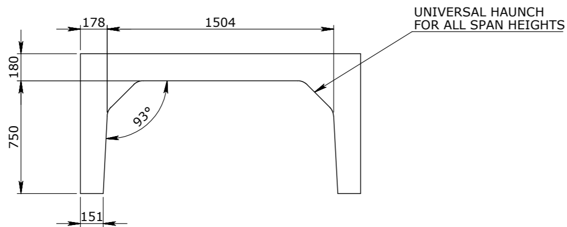
ELEVATION VIEW
