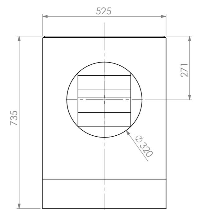
SECTION Y-Y
