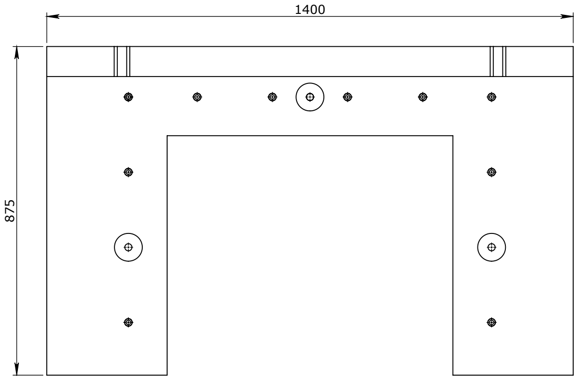
PLAN VIEW
