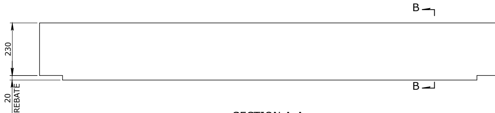
SECTION A-A SCALE 1:10
