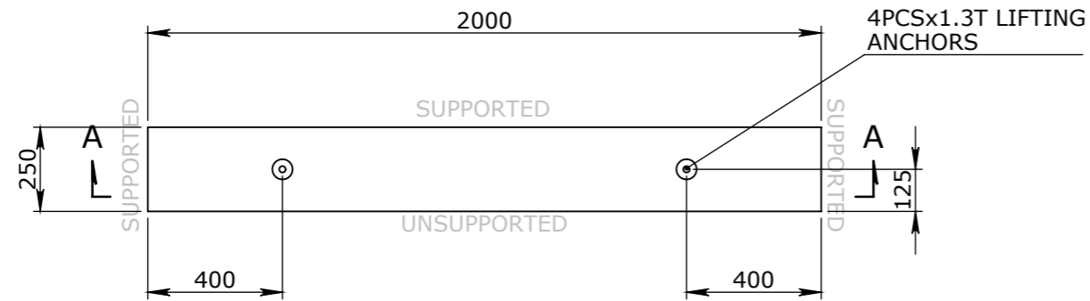
PLAN VIEW
