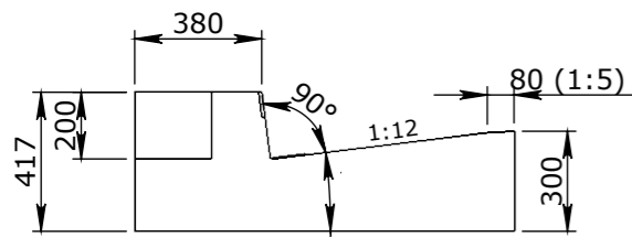
END VIEW
