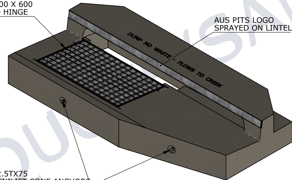
ISOMETRIC VIEW
