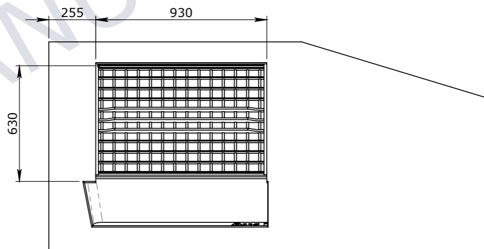
UNDERSIDE VIEW
