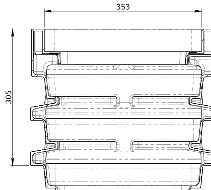
SECTION B-B
