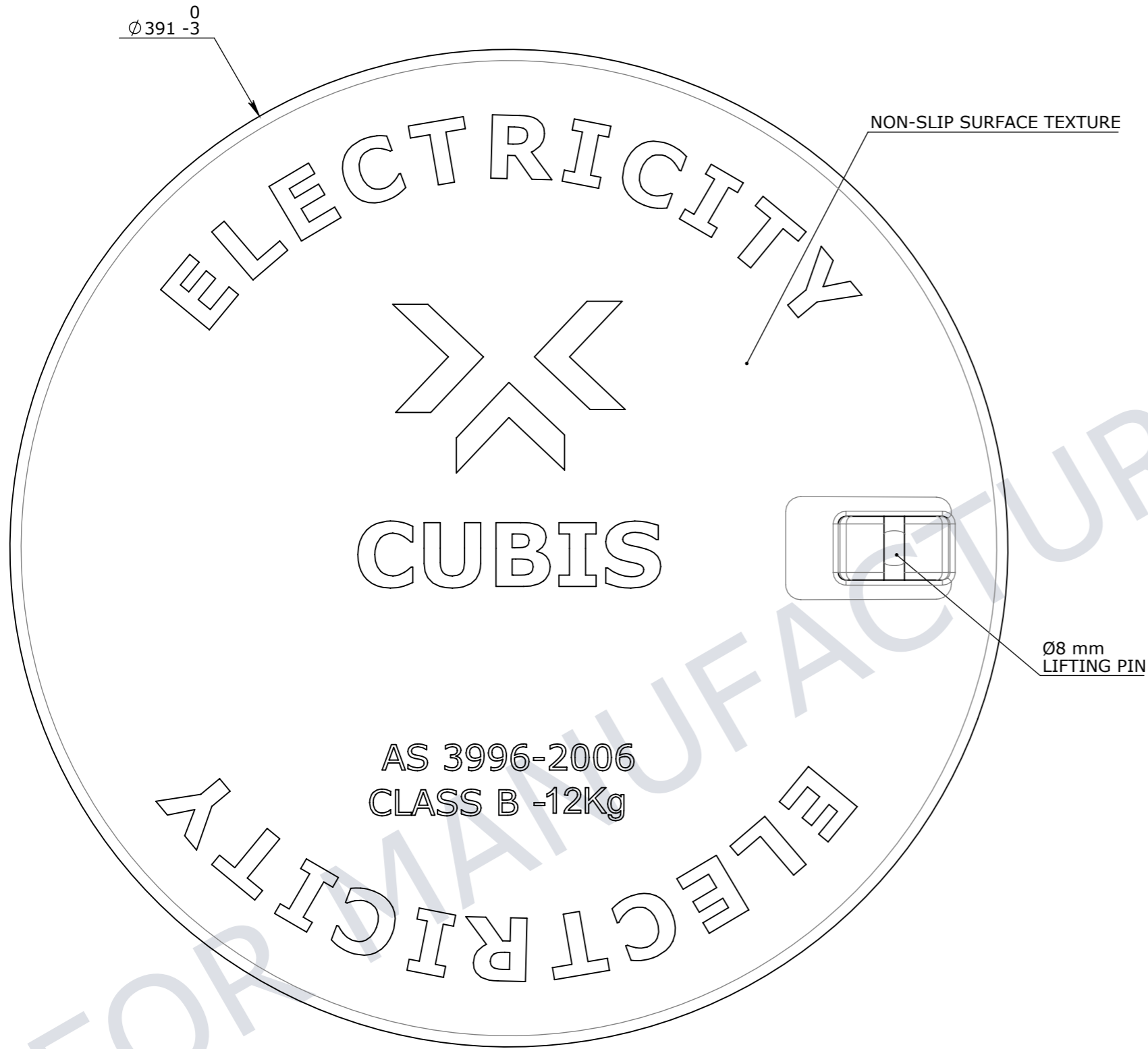
PLAN VIEW
