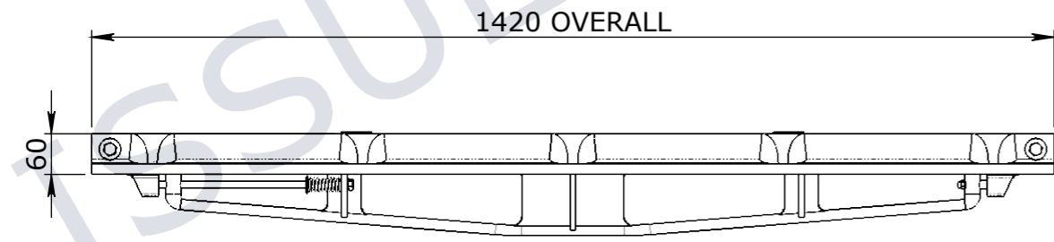
ELEVATION VIEW
