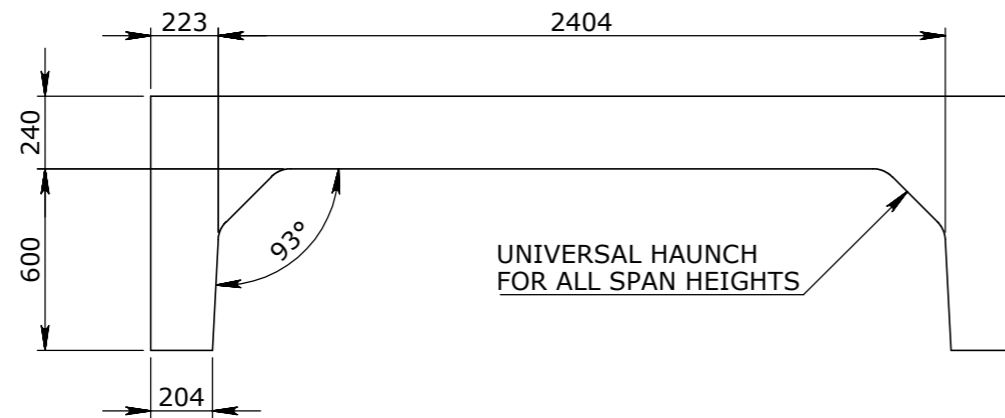
ELEVATION VIEW
