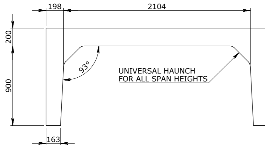
ELEVATION VIEW
