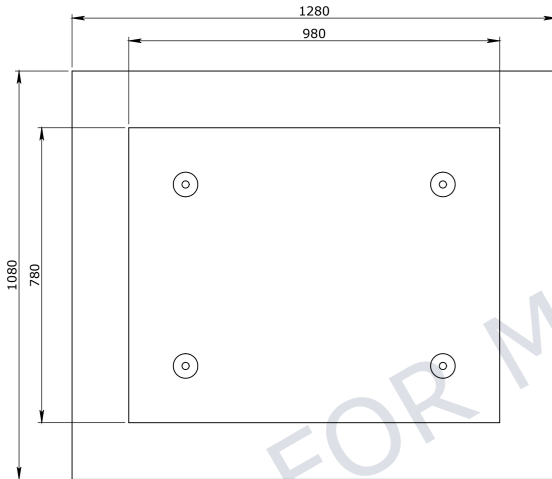
PLAN VIEW
