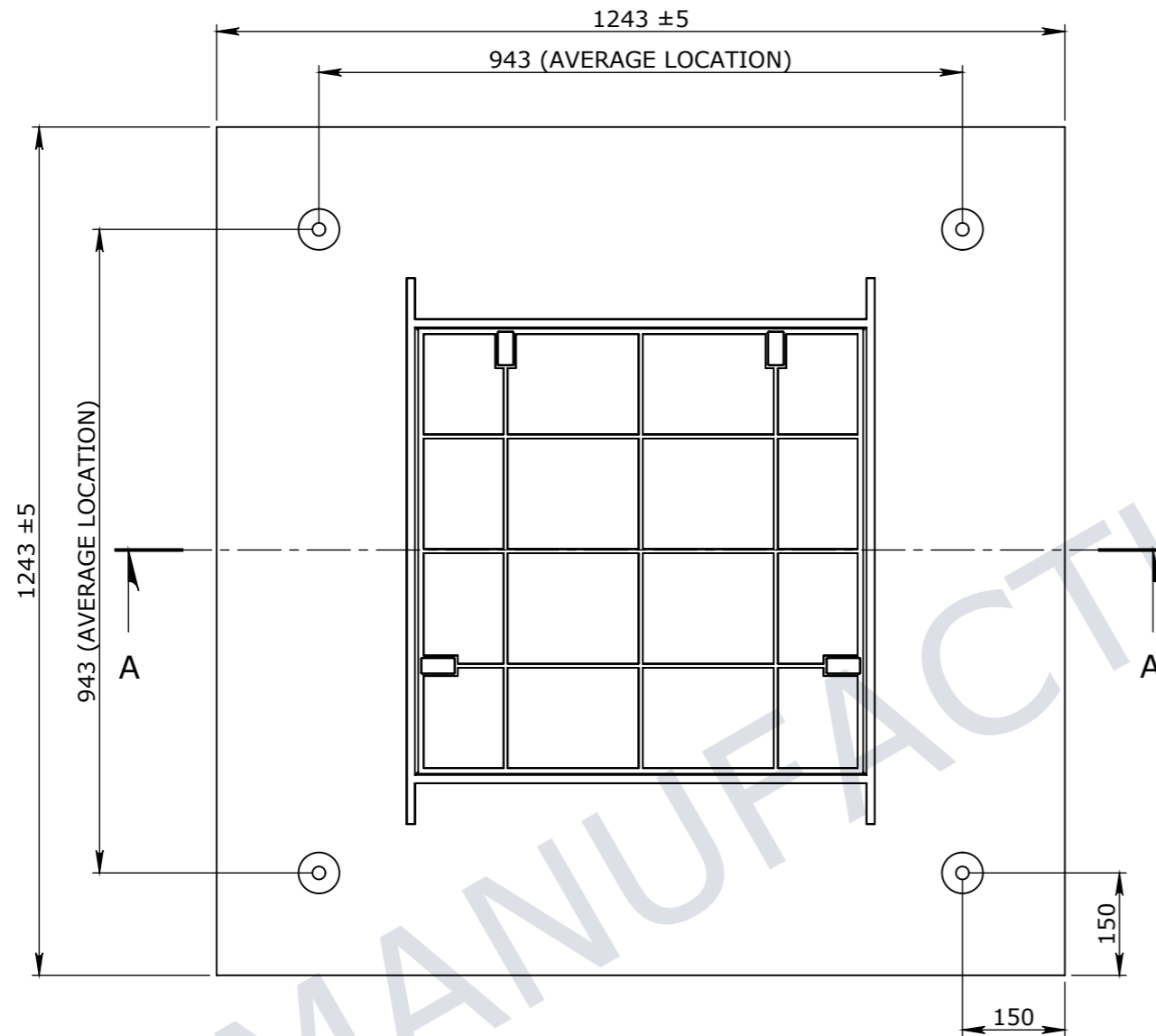
PLAN VIEW
