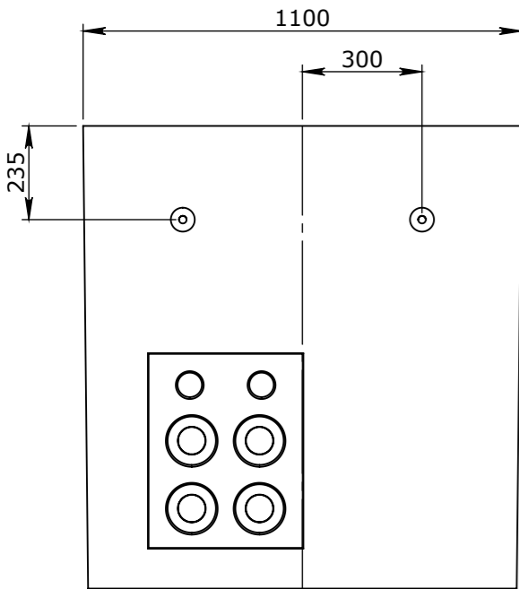
WEST FACE
