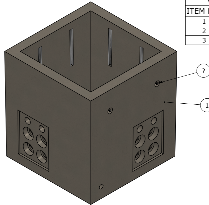
ISOMETRIC VIEW
