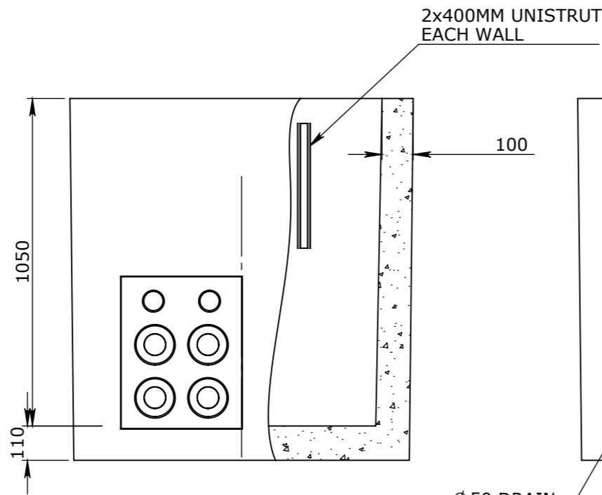
SOUTH FACE
