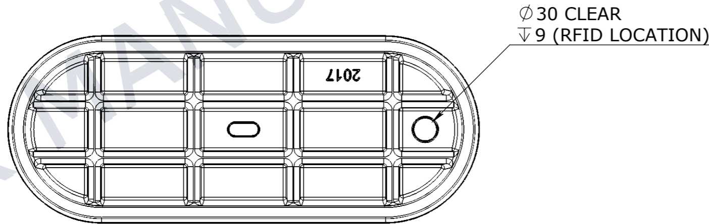
BOTTOM VIEW
