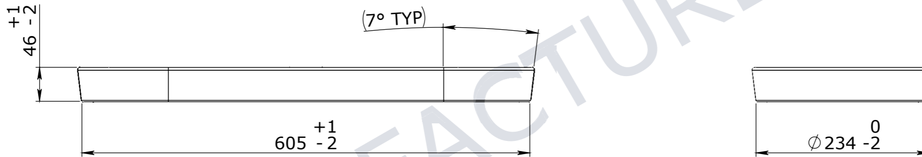
ELEVATION VIEW
