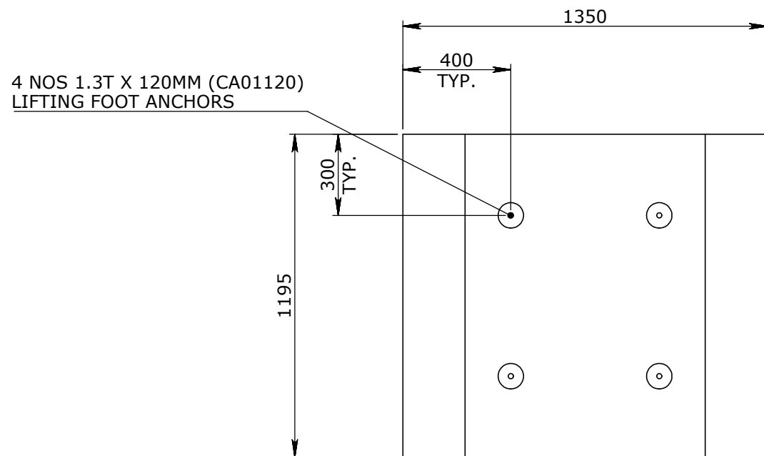
PLAN VIEW SCALE_1:20
