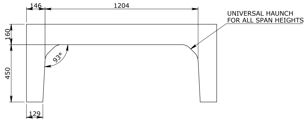
ELEVATION VIEW SCALE_1:15
