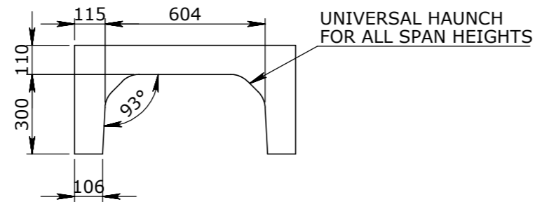
ELEVATION VIEW SCALE_1:20
