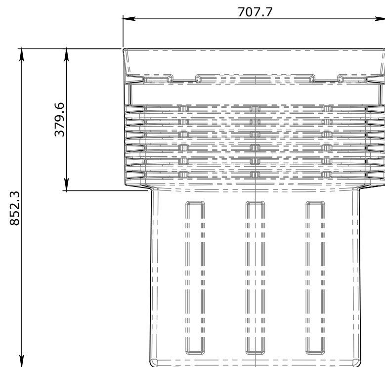
ELEVATION VIEW
